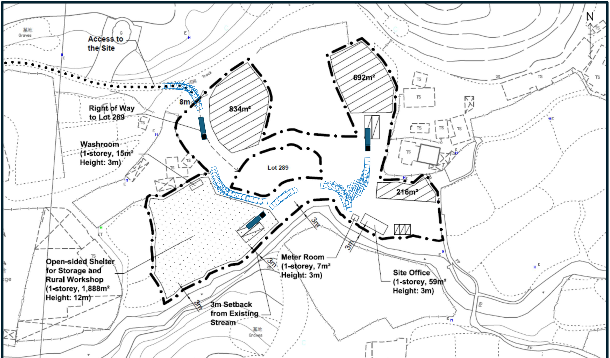
Figure 6 Swept Path Analysis Scale 1:1000
